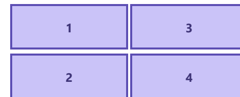
NumOfProducts: All
